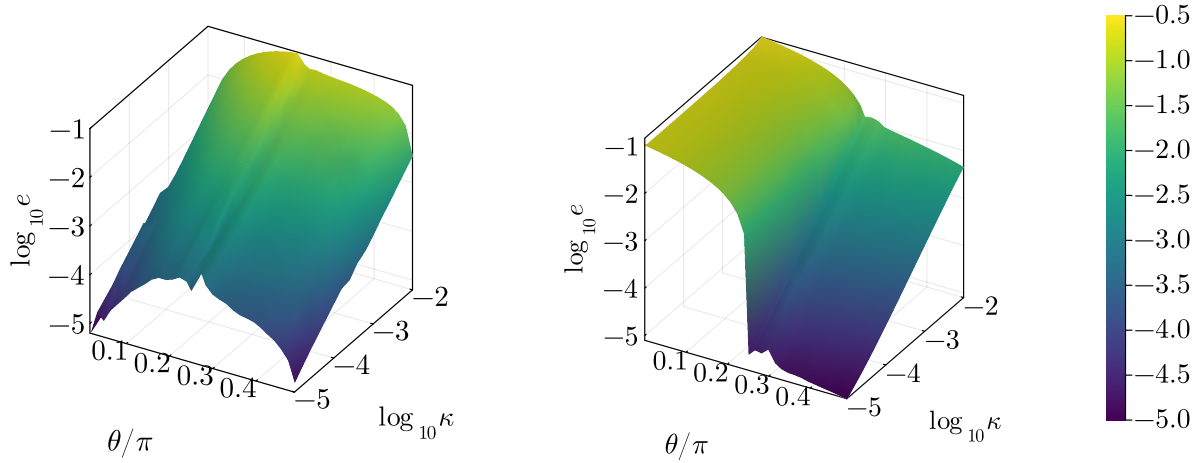
Figure 6. Optimal relative energies e_{\text{opt}}^{\text{cool}} and e_{\text{opt}}^{\text{QAOA}} as a function of \theta/\pi and \log_{10} \kappa for N = 20 with 20 free parameters. Left: optimized cooling with coupling range r_c = 1.5 and two cooling cycles. Right: QAOA with p = 10 layers. Both algorithms use as initial state \rho^{\text{cool}}(\pi/2) . The color bar applies to both panels. Cooling achieves lower energies in the topological phase ( \theta \lesssim \pi/4 ), while QAOA performs comparably or better in the trivial phase ( \theta \gtrsim \pi/4 ). Panel (d) of figure 2 shows the same optimized data as a two-dimensional heatmap.
