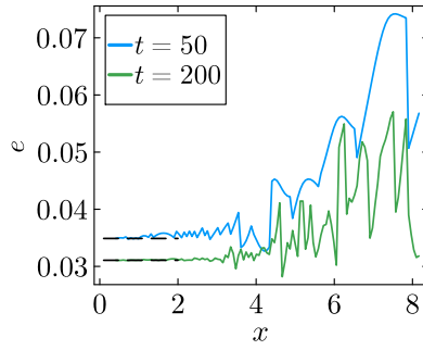
Figure 8. Relative energy e as a function of the spacing parameter x for cycle times t \in \{50, 200\} , computed by exact numerical simulation ( N = 20 , g = 10^{-3} , \kappa = 0.1g^2 , \theta = \pi/8 , \Delta_{M(m)} = \epsilon_{M(m)} \pm 0.1 ). For x \lesssim 1 , all curves reach a plateau consistent with the prediction of eq. (A.39), represented by the black dashed lines in the figure. The jagged features at larger x arise because the number of frequencies R changes discretely: each unit increase in R produces a jump in the averaged cooling rate.
