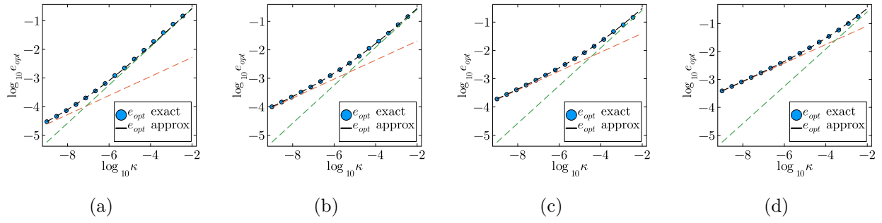
Figure 10. Optimal relative energy e_{\text{opt}}^{\text{cool}} versus noise strength \kappa (both log scale) for N = 100 , gt = 0.5 , and \Delta_{M(m)} = \epsilon_{M(m)} \pm f(\theta) in our cooling protocol. Blue circles: exact numerical optimization over t . Dashed black lines: combined approximation from eq. (A.53). Dashed green lines: multifrequency scaling \propto \kappa^{1/3} . Dashed orange lines: single-frequency scaling \propto \kappa^{2/3} . (a) \theta = \pi/1000 : the single-frequency term dominates. (b) \theta = \pi/100 : both terms contribute. (c) \theta = \pi/50 : multifrequency term begins to dominate. (d) \theta = \pi/20 : the \kappa^{1/3} many-frequency scaling holds over most of the range.
