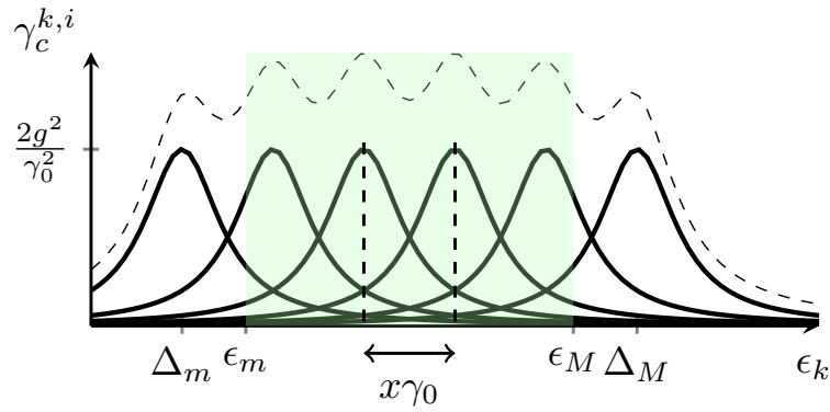
Figure 3. Individual cooling rates \gamma_c^{k,i} (Lorentzian profiles) and their sum \tilde{\gamma}_k^c (dashed curve) as a function of the mode energy \epsilon_k for a set of bath frequencies \{\Delta_r\} equally spaced over the interval [\Delta_m, \Delta_M] . The spacing between two adjacent frequencies is x\gamma_0 , where x is a dimensionless parameter and \gamma_0 \propto 1/t is the Lorentzian linewidth. Each frequency generates a resonance peak of width \gamma_0 centered at \epsilon_k = \Delta_r and height 2g^2/\gamma_0^2 . When the peaks overlap sufficiently ( x \lesssim 1 ), the averaged cooling rate \gamma_k^c becomes approximately independent of k , ensuring uniform cooling of all modes in the range [\epsilon_m, \epsilon_M] (green area).
