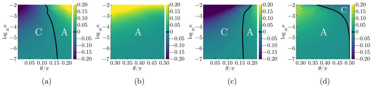
Figure 1. Difference e_{\text{opt}}^{\text{cool}} - e_{\text{opt}}^{\text{adiab}} between the optimal relative energies achieved by the cooling and the adiabatic algorithms, plotted as a function of \theta/\pi (horizontal axis) and \log_{10} \kappa (vertical axis) for N = 100 systems. Negative values (blue/dark) indicate that cooling gives lower energy (region labeled “C”); positive values (yellow/bright) indicate that the adiabatic algorithm gives lower energy (region labeled “A”). The black contour marks e_{\text{cool}}^{\text{opt}} = e_{\text{adiab}}^{\text{opt}} . (a) Topological phase, adiabatic algorithm starting from |0\rangle^{\otimes N} (ideal): cooling gives lower energy throughout most of this phase. (b) Trivial phase, ideal adiabatic algorithm: the adiabatic algorithm gives lower energy everywhere due to its small non-adiabatic prefactor and the \kappa^{2/3} power law in this gapped regime. (c) Topological phase, realistic adiabatic algorithm starting from \rho^{\text{cool}}(\pi/2) : the region where cooling yields lower energy expands. (d) Trivial phase, realistic adiabatic: the imperfect initial state reduces the adiabatic advantage, and cooling yields lower energy for \kappa \gtrsim 10^{-3} . For cooling the relative energies are computed numerically at N = 100 , whereas for relative energies achieved by the adiabatic algorithm we use the large- N analytic formulas to suppress the finite-size effect. The deviations at high \kappa are due to the fact that we enter a regime where the here chosen discretization of R matters (see appendix A.4).
