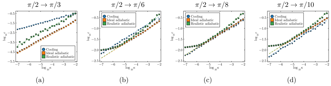
Figure 4. Optimal relative energy e_{\text{opt}} (log scale) as a function of the noise strength \kappa (log scale) for N = 100 sites, comparing three protocols: analytic cooling with gt = 0.5 and \Delta_{M(m)} = \epsilon_{M(m)} \pm 0.4 (blue circles), ideal adiabatic with initial state |0\rangle^{\otimes N} (orange squares), and realistic adiabatic with initial state \rho^{\text{cool}}(\pi/2) (green squares). Dashed lines show the analytic predictions from eq. (5.1) (blue, \kappa^{1/3} ) and appendix B (orange, green). (a) \theta_f = \pi/3 (trivial phase): the adiabatic \kappa^{2/3} scaling gives lower energy than the achievable rate of the cooling algorithm, which is \kappa^{1/3} . (b) \theta_f = \pi/6 (topological phase): both scale as \kappa^{1/3} ; the adiabatic algorithm gives slightly lower energy. (c) \theta_f = \pi/8 : the two algorithms become comparable. (d) \theta_f = \pi/10 : cooling gives lower energy than both adiabatic protocols. In panels (b)–(d), the adiabatic curves flatten at small \kappa due to the unavoidable excitation of the zero-gap mode k = N/2 .
