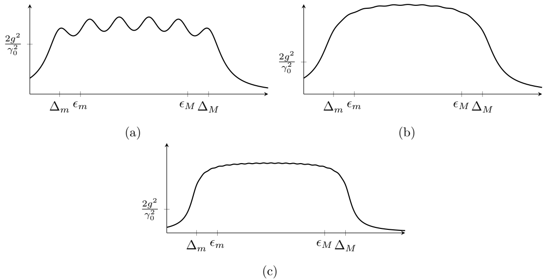
Figure 7. Rescaled averaged cooling rate R\gamma_k^c versus mode energy \epsilon_k for three configurations of bath frequencies. The interval [\epsilon_m, \epsilon_M] marks the system's spectral range; [\Delta_m, \Delta_M] marks the bath frequency range. (a) Too few frequencies: pronounced peaks and valleys lead to strongly non-uniform cooling. (b) Sufficiently many frequencies but short cycle times (broad linewidth \gamma_0 ): resonance peaks extend well beyond the spectrum. (c) Many frequencies with long cycle times (narrow linewidth): the averaged rate is approximately flat across [\epsilon_m, \epsilon_M] and decays sharply outside, yielding the desired uniform cooling profile.
