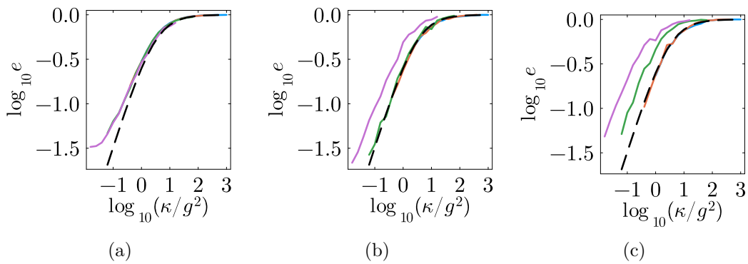
Figure 9. Relative energy e versus the ratio \kappa/g^2 for cooling with three cycle times: (a) t = 10 , (b) t = 50 , (c) t = 100 , and four coupling strengths g = 0.003 (blue), 0.005 (orange), 0.013 (green), 0.025 (purple). The dashed black line shows the analytic prediction from eq. (A.42). Agreement is good when \kappa/g^2 \gtrsim 1 and gt \lesssim 0.5 ; deviations at smaller \kappa/g^2 or larger gt indicate breakdown of the long-time or weak-coupling approximations. Parameters: N = 20 , \theta = \pi/8 , \Delta_{M(m)} = \epsilon_{M(m)} \pm 0.1 .
