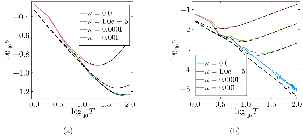
Figure 11. Relative energy e versus total evolution time T (log-log scale) for adiabatic evolution targeting (a) \theta_f = \pi/8 and (b) \theta_f = \pi/3 at several noise rates \kappa , for system size N = 20 . Solid lines: exact numerical simulation. Dashed lines: analytic predictions. In the presence of noise, each curve exhibits a minimum at an optimal T , reflecting the trade-off between non-adiabatic excitations and depolarizing noise. For larger T , the energy increases as noise effects dominate. The analytical predictions accurately capture both the scaling behavior and the position of these minima.
