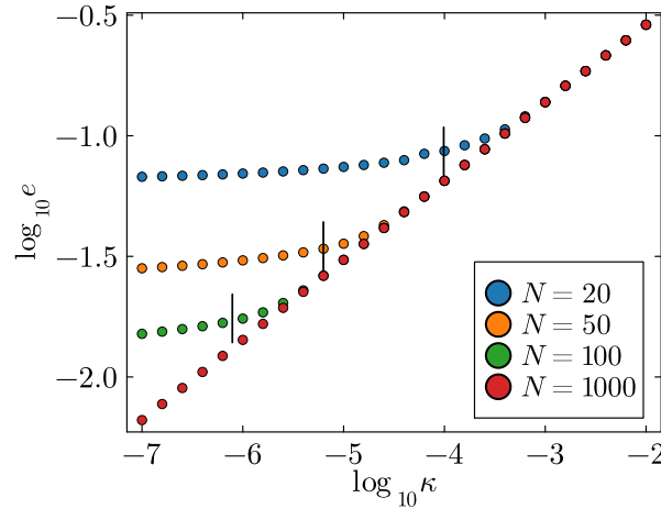
Figure 5. Optimal relative energy e_{\text{opt}}^{\text{adiab}} as a function of the noise rate \kappa for different system sizes N and target \theta_f = \pi/10 for the ideal adiabatic algorithm. The smaller the system size, the more prominent the effect of the k = N/2 mode is, and the larger the \kappa_{\text{min}} where the crossover (predicted by the vertical lines) happens. The predicted plateau values of \log_{10} e are determined by the finite-size floor 2\epsilon_{N/2}/|E_{\text{GS}}| .
