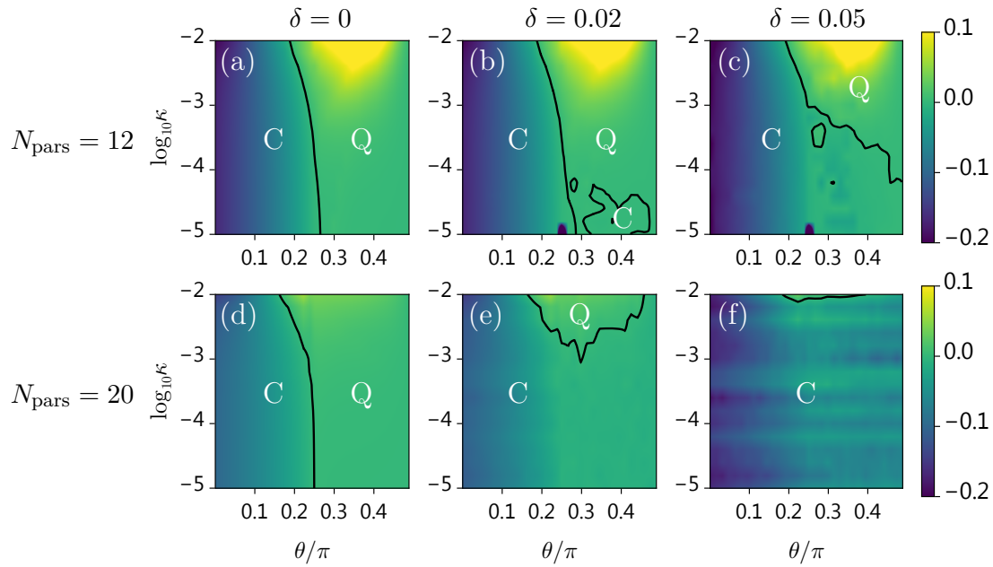
Figure 2. Difference e_{\text{opt}}^{\text{cool}} - e_{\text{opt}}^{\text{QAOA}} as a function of \theta/\pi (horizontal) and \log_{10} \kappa (vertical) for N = 20 . Blue: cooling gives lower energy (labeled “C”); yellow: QAOA gives lower energy (labeled “Q”); black contour: equal performance. Top row ( N_{\text{pars}} = 12 ): cooling with coupling range r_c = 0.5 and two cycles; QAOA with p = 6 layers. Bottom row ( N_{\text{pars}} = 20 ): r_c = 1.5 , p = 10 . Columns show increasing deviation of the exact parameters, \delta : (a, d) \delta = 0 (exact parameters); (b, e) \delta = 0.02 ; (c, f) \delta = 0.05 , each averaged over 100 random perturbations. Both algorithms start from \rho^{\text{cool}}(\pi/2) . As \delta increases, the region where cooling outperforms QAOA expands, demonstrating cooling’s greater robustness to parameter imperfections. The “islands” seen in (b, c) are caused by fluctuations in the optimal parameters in a region where both methods are almost equally effective.
