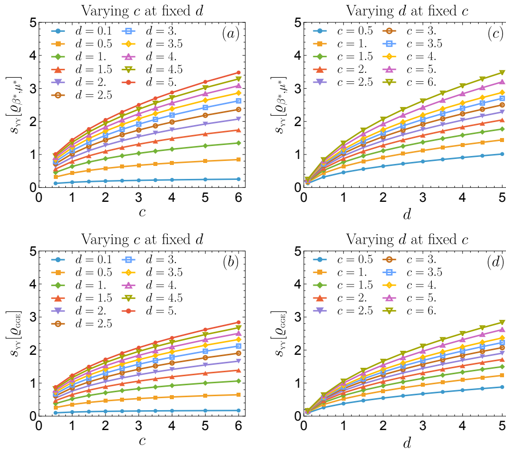
Figure 22. Thermal and GGE entropy densities for the BEC to repulsive ( c > 0 ) LL quenches associated with figure 11. (a) and (b) show, respectively, s_{YY}[\varrho_{\beta^*, \mu^*}] and s_{YY}[\varrho_{GGE}] as functions of the postquench interaction c at fixed particle density d . (c) and (d) show, respectively, s_{YY}[\varrho_{\beta^*, \mu^*}] and s_{YY}[\varrho_{GGE}] as functions of d at fixed postquench c .
