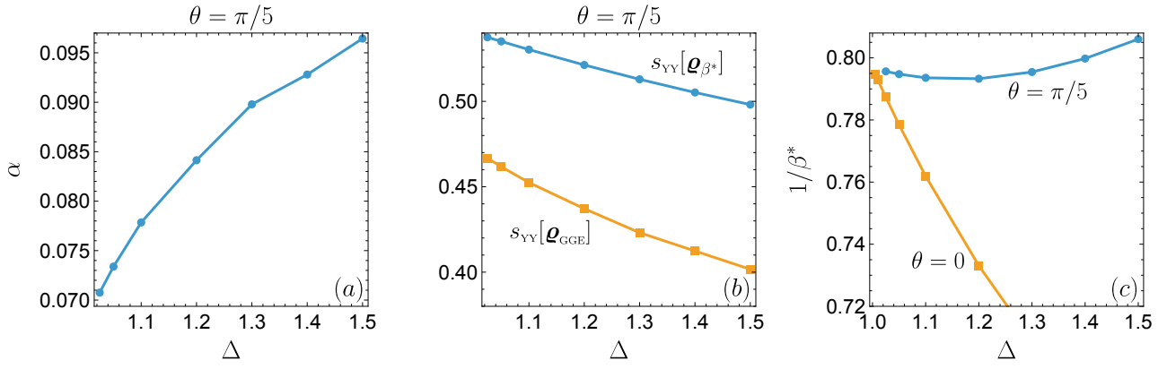
Figure 10. Density of athermality \alpha (a), GGE and GE entropy densities (b) and temperatures 1/\beta^* (c) as a function of \Delta in the quench from the tilted-Néel state (5.4) with \theta = \pi/5 . In (c) we also plot for comparison the temperature of the Néel quench ( \theta = 0 ). The continuous lines are just guides to the eye.
