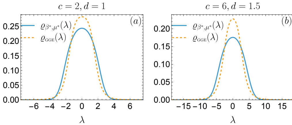
Figure 12. Comparison between \varrho_{\beta^*, \mu^*}(\lambda) (continuous line) and \varrho_{\text{GGE}}(\lambda) (dashed line) in the repulsive regime for different values of c > 0 and density of particles d .
