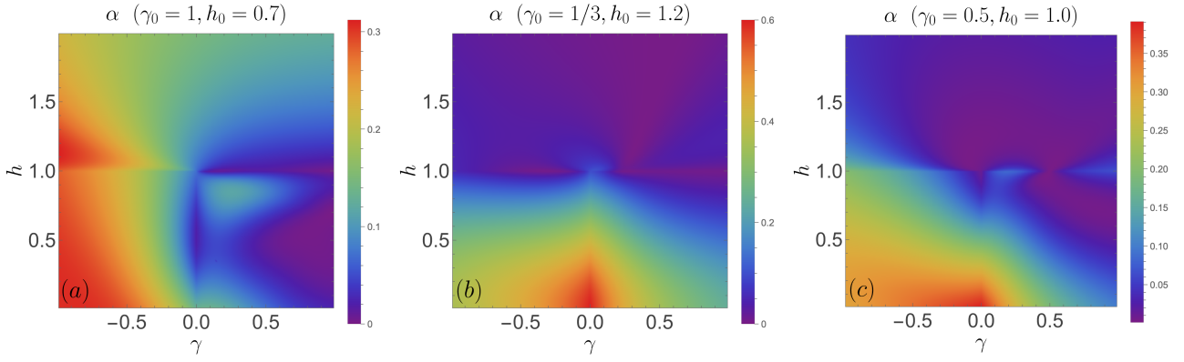
Figure 2. Density plots for the density of athermality \alpha in the plane (\gamma, h) , for fixed prequench parameters (\gamma_0, h_0) . (a) and (b) correspond to noncritical initial states, while (c) shows results for a critical initial state on the Ising line h_0 = 1 . See figure 16 in appendix C for corresponding plots for the energy density e and the entropy densities s_{\text{YY}}[\varrho_{\text{GGE}}] and s_{\text{YY}}[\varrho_{\beta^*}] .
