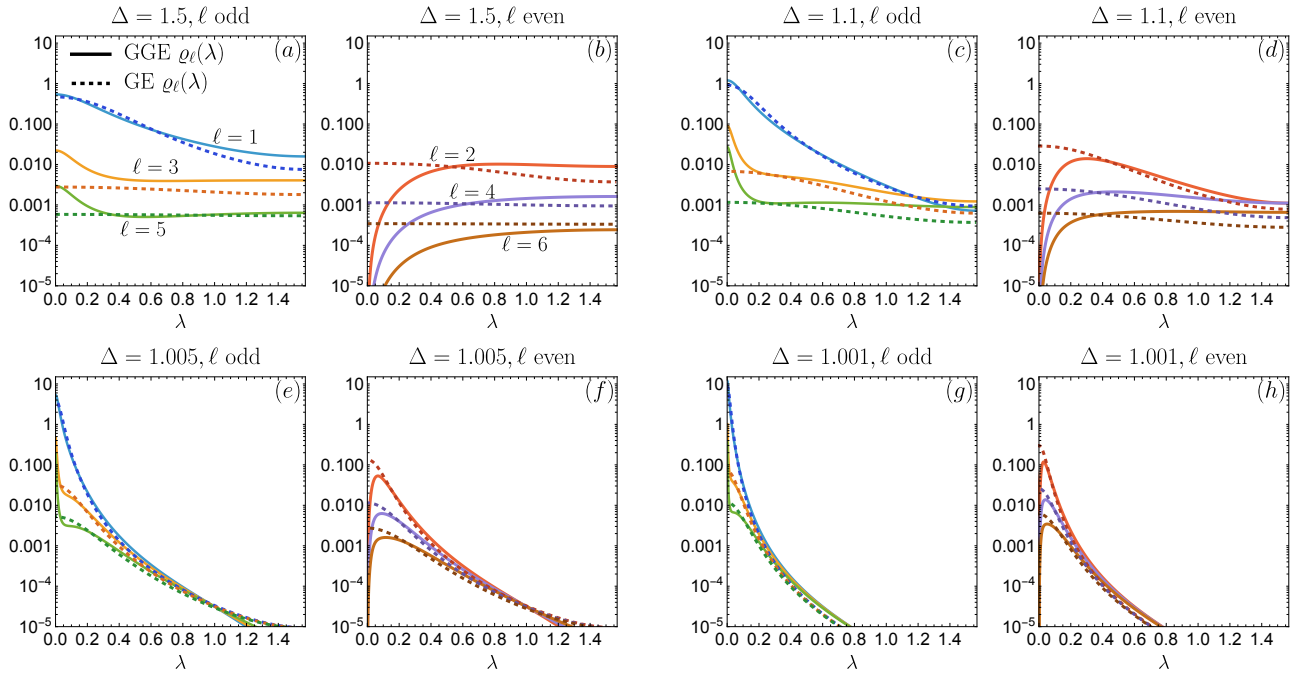
Figure 9. Log-scale plots for the GE (dashed lines) and GGE (continuous lines) root densities \varrho_\ell(\lambda) for 1 \leq \ell \leq 6 and \Delta > 1 in the Néel quench ( \theta = 0 ). The curves are shown only for \lambda \geq 0 as they are symmetric around \lambda = 0 .
