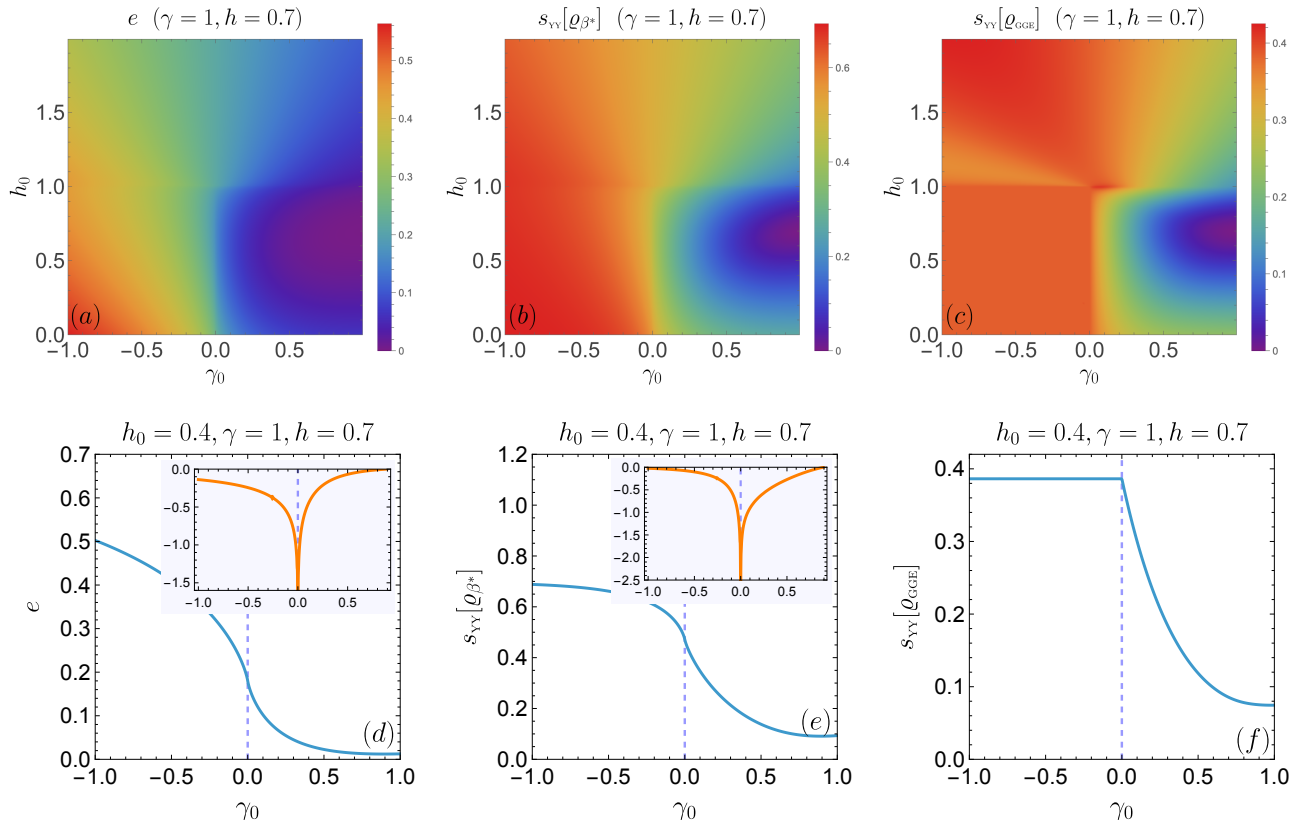
Figure 18. Density plots and cuts for e , s_{\text{YY}}[Q_{\beta^*}] and s_{\text{YY}}[Q_{\text{GGE}}] , associated with the athermality plots of figure 7(a). The subplots (d), (e) and (f) correspond, respectively, to horizontal cuts in the density subplots (a), (b) and (c). Insets in (d) and (e) show numerically computed derivatives of the curves in the main plot. In computing the energy density e we set E_e and E_o from equation (4.2) to zero.
