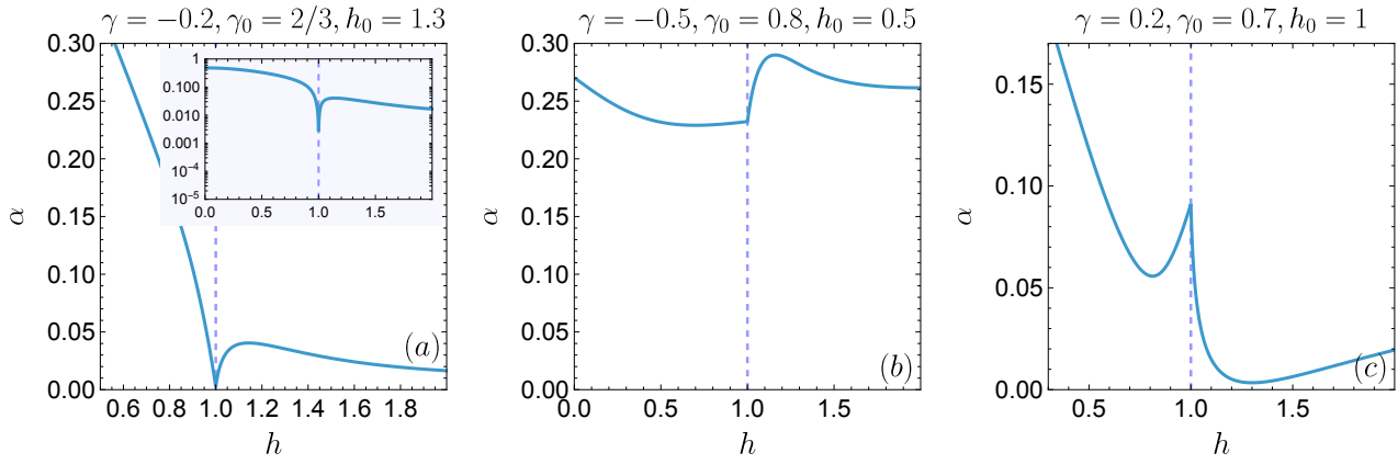
Figure 4. \alpha as a function of h , for fixed \gamma \neq \gamma_0 ( h - and \gamma -driven quench) and h_0 . The blue dashed lines indicates the critical Ising point h = 1 . The inset in (a) shows the same data in log-scale.
