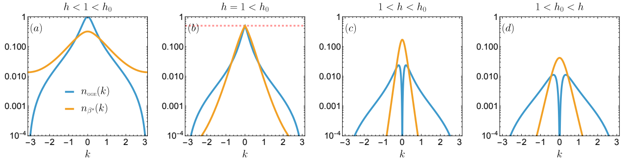
Figure 17. Log-scale comparison between the occupation functions n_{\text{GGE}}(k) and n_{\beta^*}(k) , for different choices of h in the TFIC ( \gamma = \gamma_0 = 1 ) with h_0 = 1.3 : (a) h = 0.7 ; (b) h = 1 (critical), with red dashed line indicates the pinning at 1/2 ; (c) h = 1.15 ; (d) h = 1.5 .
