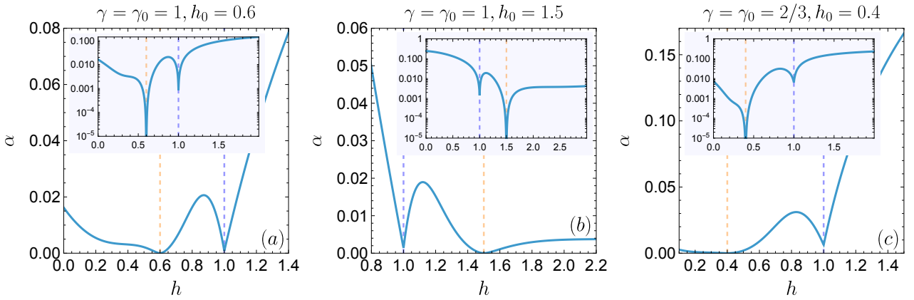
Figure 3. Density of athermality \alpha as a function of the postquench transverse field h , for fixed \gamma = \gamma_0 ( h -driven quench) and h_0 . The orange and blue dashed lines indicate, respectively, the trivial zero at h = h_0 and the critical Ising point h = 1 . (a) and (b) correspond to quenches in the TFIC ( \gamma = \gamma_0 = 1 ), while in (c) the anisotropy is present. Insets: same data in log-scale.
