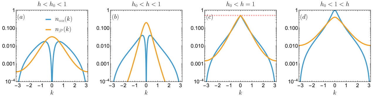
Figure 6. Log-scale comparison between the occupation functions n_{\text{GGE}}(k) and n_{\beta^*}(k) , for different choices of h in the TFIC ( \gamma = \gamma_0 = 1 ) with h_0 = 0.6 : (a) h = 0.4 ; (b) h = 0.8 ; (c) h = 1 (critical), with red dashed line indicating the pinning value of 1/2 ; (d) h = 1.2 .
