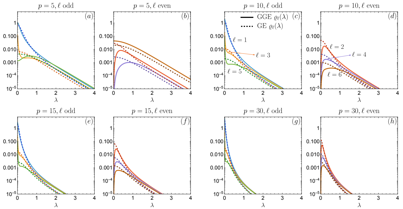
Figure 19. Log-scale plots for the GE (dashed lines) and GGE (continuous lines) root densities \varrho_\ell(\lambda) for 1 \leq \ell \leq 6 and for a few values of 0 < \Delta < 1 in the Néel quench ( \theta = 0 ). The integer p refers to the parametrization (5.2) of the anisotropy \Delta , with p \rightarrow \infty corresponding to the critical limit \Delta \rightarrow 1 .
