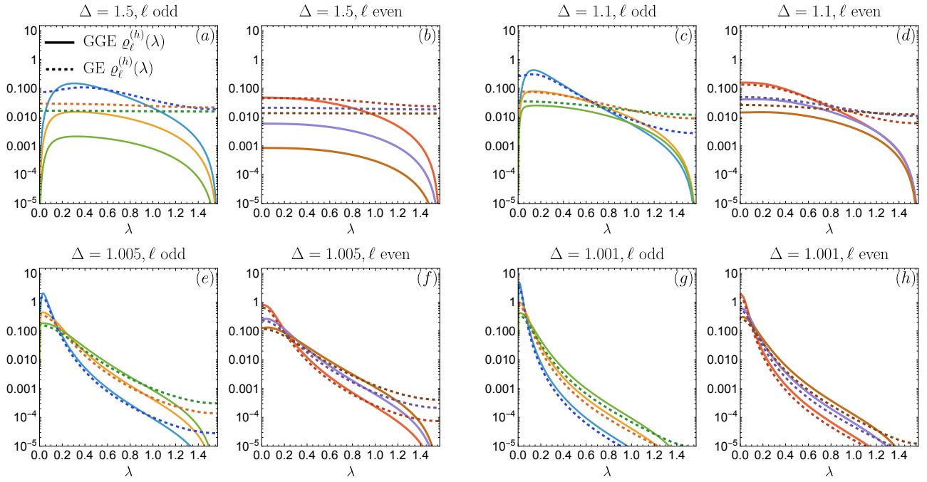
Figure 20. Log-scale plots for the GE (dashed lines) and GGE (continuous lines) hole densities \varrho_\ell^{(h)}(\lambda) for 1 \leq \ell \leq 6 and \Delta > 1 in the Néel quench ( \theta = 0 ). The color scheme is the same as previous figures, i.e. \ell = 1, 3, 5 corresponding to blue, orange, green and \ell = 2, 4, 6 to red, purple, brown.
