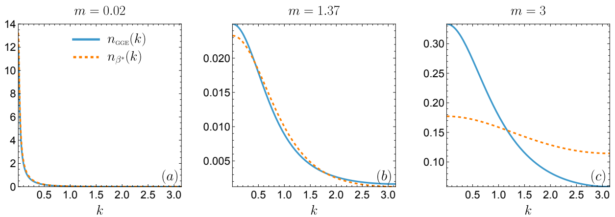
Figure 15. GGE and thermal occupation functions n_{\text{GGE}}(k) and n_{\beta^*}(k) for a few values of the postquench mass m in the quench from the GS with m_0 = 1 . (a) m = 0.02 close to criticality; (b) m = 1.37 , corresponding to the non-trivial minimum in the athermality of figure 14(a); (c) m = 3 .
