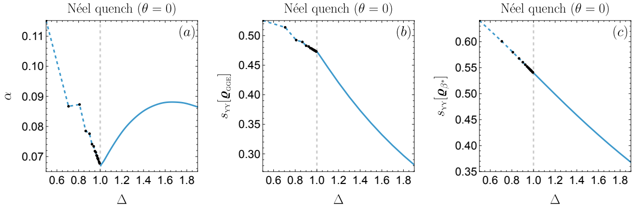
Figure 8. Densities of athermality \alpha (a), GGE entropy s_{YY}[\varrho_{GGE}] (b) and GE entropy s_{YY}[\varrho_{\beta^*}] (c) as a function of \Delta in the quench from the Néel state (equation (5.4) for \theta = 0 ). The dashed blue lines in the interval 0 < \Delta < 1 are just guides to the eye that connect results for the anisotropies in equation (5.2). The vertical dashed line indicates the critical point \Delta = 1 .
