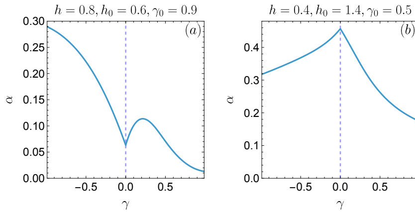
Figure 5. \alpha as a function of \gamma , for fixed h \neq h_0 ( h - and \gamma -driven quench) and \gamma_0 . The blue dashed lines indicates the critical XX point \gamma = 0 .
