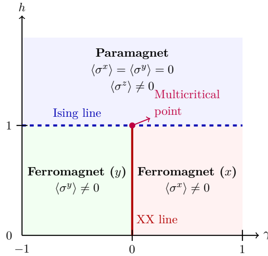
Figure 1. T = 0 quantum phase diagram of the XY chain in a transverse field with Hamiltonian H_{XY}(\gamma, h) from equation (4.1). See text for description of (i) Ising critical line (blue dashed) and (ii) XX critical line (red).
