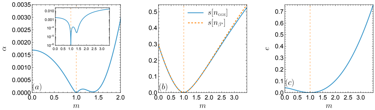
Figure 14. Densities of athermality \alpha (a), GGE and GE entropy (b) and energy e (c) as a function of m in the quench from the GS with m_0 = 1 . The vertical dashed lines indicate the position of the trivial zero m = m_0 . The inset in (a) shows the same data in log-scale.
