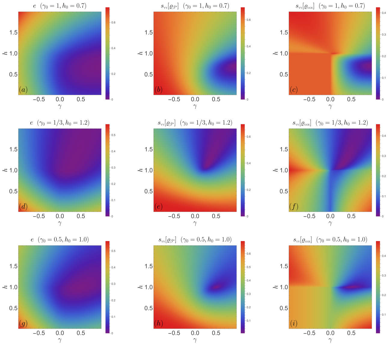
Figure 16. Density plots for e , s_{YY}[\rho_{\beta^*}] and s_{YY}[\rho_{GGE}] , associated with the athermality plots of figure 2. (a)-(c) Subplots associated with figure 2(a). (d)-(f) Subplots associated with figure 2(b). (g)-(i) Subplots associated with figure 2(c). In computing the energy density e we have set the ground state energies E_e and E_o from equation (4.2) to zero.
