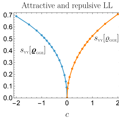
Figure 13. GGE entropy density for repulsive c > 0 ( s_{\text{YY}}[\varrho_{\text{GGE}}] ) and attractive c < 0 ( s_{\text{YY}}[\varrho_{\text{GGE}}] ) interactions in the LL quench from the BEC state (6.3) with density of particles d = 1 . The point c = 0 corresponds a trivial zero due to absence of the quench.
