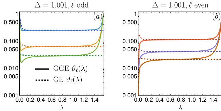
Figure 21. Log-scale plots for the GE (dashed lines) and GGE (continuous lines) filling functions \vartheta_\ell(\lambda) = \varrho_\ell(\lambda)/\varrho_\ell^{(\text{tot})}(\lambda) for 1 \leq \ell \leq 6 (same color scheme as above) and \Delta = 1.001 in the Néel quench ( \theta = 0 ).
