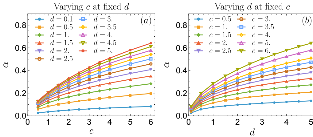
Figure 11. Density of athermality \alpha associated with the BEC-to-repulsive-LL quench. (a) \alpha as a function of the postquench interaction c > 0 at fixed particle density d . (b) \alpha as a function of d at fixed postquench c .
