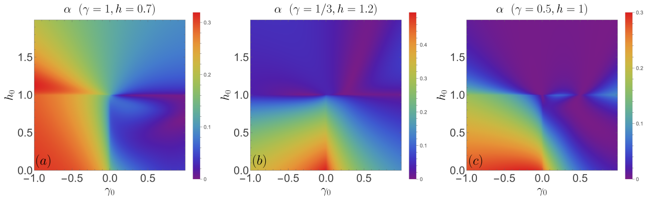
Figure 7. Density plots for \alpha in the plane (\gamma_0, h_0) , for fixed postquench parameters (\gamma, h) . The subplots (a), (b) and (c) correspond to the (a), (b) and (c) density subplots of figure 2 under the swap (\gamma, h) \leftrightarrow (\gamma_0, h_0) . In particular, current subplot (c) corresponds to a quench to a critical Hamiltonian on the Ising line.
