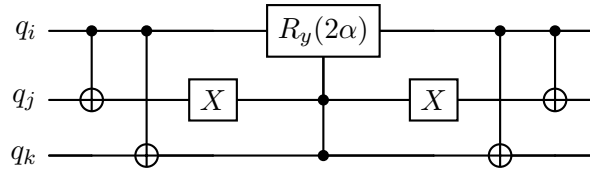
Figure 6. Decomposition of the BEMPA \hat{B} gate. The CNOT cascade controlled by q_i maps |001\rangle and |110\rangle to states differing only in q_i . The X gate on q_j isolates these two states so that only they trigger the C^2 R_y(2\alpha) rotation on q_i .
