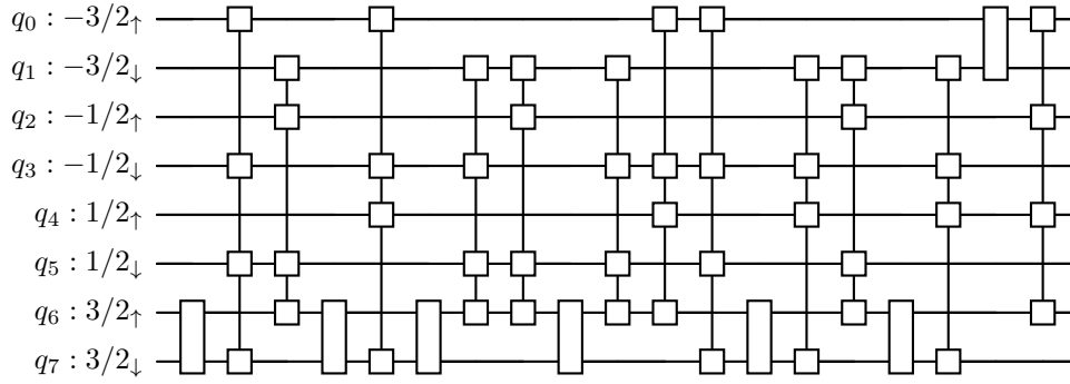
Figure 1. A 19-parameter G -gate circuit that is numerically surjective on the S_z = 0 subspace for N = 4 , starting from the input state |01010101\rangle . The first 17 gates form a minimal spanning circuit of G^{(2)} gates on the (q_6, q_7) isospin pair interleaved with various G^{(4)} gates; the two additional gates G_{01}^{(2)} and G_{0624}^{(4)} close the local-to-global gap, so that numerical optimisation reaches every tested random target on S^{17} .
