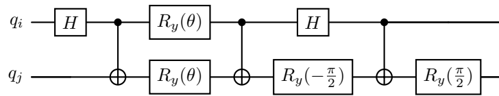
Figure 5. Minimal exact decomposition of the 2-qubit A -gate A_{ij}^{(2)}(\theta) into three CNOT gates. The first two CNOTs implement G(-\theta) as in figure 4 (note the sign change from R_y(-\theta) to R_y(\theta) , which reverses the rotation direction), and the third implements the reflection A(0) .
