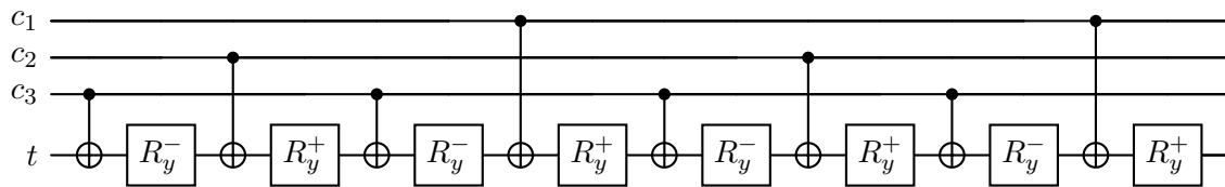
Figure 9. Decomposition of C^3 R_y(\alpha) into 8 CNOT gates and 8 single-qubit rotations R_y^\pm \equiv R_y(\pm\alpha/8) of alternating sign. The CNOT controls follow the Gray code pattern c_3, c_2, c_3, c_1, c_3, c_2, c_3, c_1 , where c_3 toggles most frequently. The same pattern with two controls and 4 CNOTs gives C^2 R_y(\alpha) with R_y(\pm\alpha/4) .
