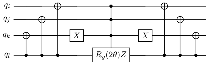
Figure 8. Decomposition of the 4-qubit A -gate A_{ijkl}^{(4)}(\theta) . The CNOT cascade is identical to figure 7. The multi-controlled gate on q_l applies C^3(R_y(2\theta)Z) combined with a C^3(-I) phase correction to implement the reflection A^{(4)}(0) together with G^{(4)}(-\theta) . In practice, the overall C^3(-I) can be absorbed into the decomposition of the multi-controlled gate.
