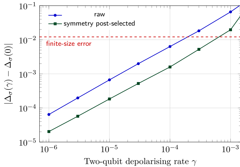
Figure 3. Noise-induced error on the extracted scaling dimension \Delta_\sigma as a function of the two-qubit depolarising rate \gamma , for N = 4 . The dashed line is the finite-size error |\Delta_\sigma(0) - \Delta_\sigma^{\text{bootstrap}}| = 1.21 \times 10^{-2} . The noise-induced error grows essentially linearly in \gamma and crosses the finite-size error at \gamma \approx 2.0 \times 10^{-4} for the raw estimator, and at \gamma \approx 6.5 \times 10^{-4} after symmetry post-selection.
