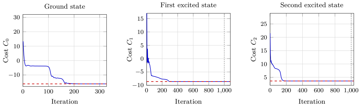
Figure 2. VQE/VQD convergence for the three lowest eigenstates of the fuzzy sphere Hamiltonian ( N = 4 ). Each panel shows the cost function at every iteration (blue curve), with the exact eigenvalue from ED indicated by the red dashed line. For the excited states (centre and right panels), the dotted vertical line marks the transition from the Adam phase to the gradient-descent phase.
