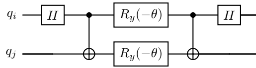
Figure 4. Decomposition of the 2-qubit Givens rotation G_{ij}^{(2)}(\theta) into two CNOT gates and single-qubit rotations.
