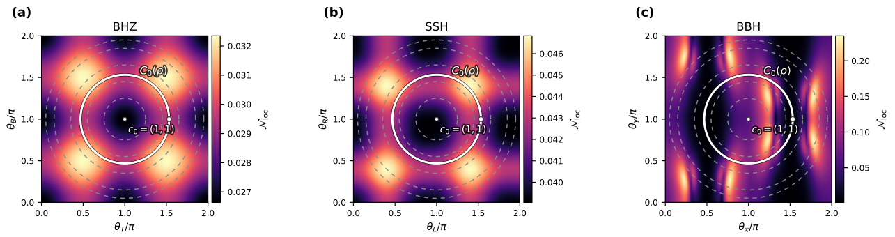
Figure 6. Contractible center-based family on the control tori. The same center c_0 = (1, 1) and radius scan \mathcal{C}_0(\rho) are used in BHZ, SSH and BBH. Dashed curves show the scanned radii; the solid curve marks the benchmark circle \rho = 0.53 used for the orientation check. The heat maps show refined link-level distances \mathcal{N}_{\text{loc}} , plotted with periodic edge filling to avoid artificial blank boundaries.
