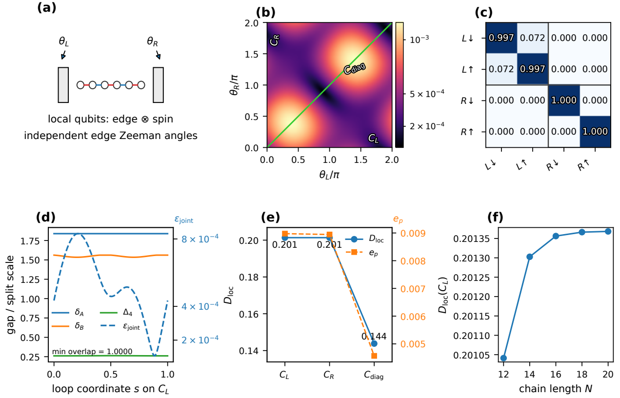
Figure 3. SSH benchmark. (a) Open spinful SSH chain with independent edge angles (\theta_L, \theta_R) . (b) \epsilon_{\text{joint}} map on the edge-angle torus, with representative loops overlaid. (c) Left-loop holonomy in the extracted local basis. (d) Along-loop quality on C_L . (e) Representative loop comparison, shown as aligned D_{\text{loc}} and entangling-power e_p axes. (f) Finite-size dependence of the single-edge response. Supplementary scans display nearby branches, including the anti-diagonal family.
