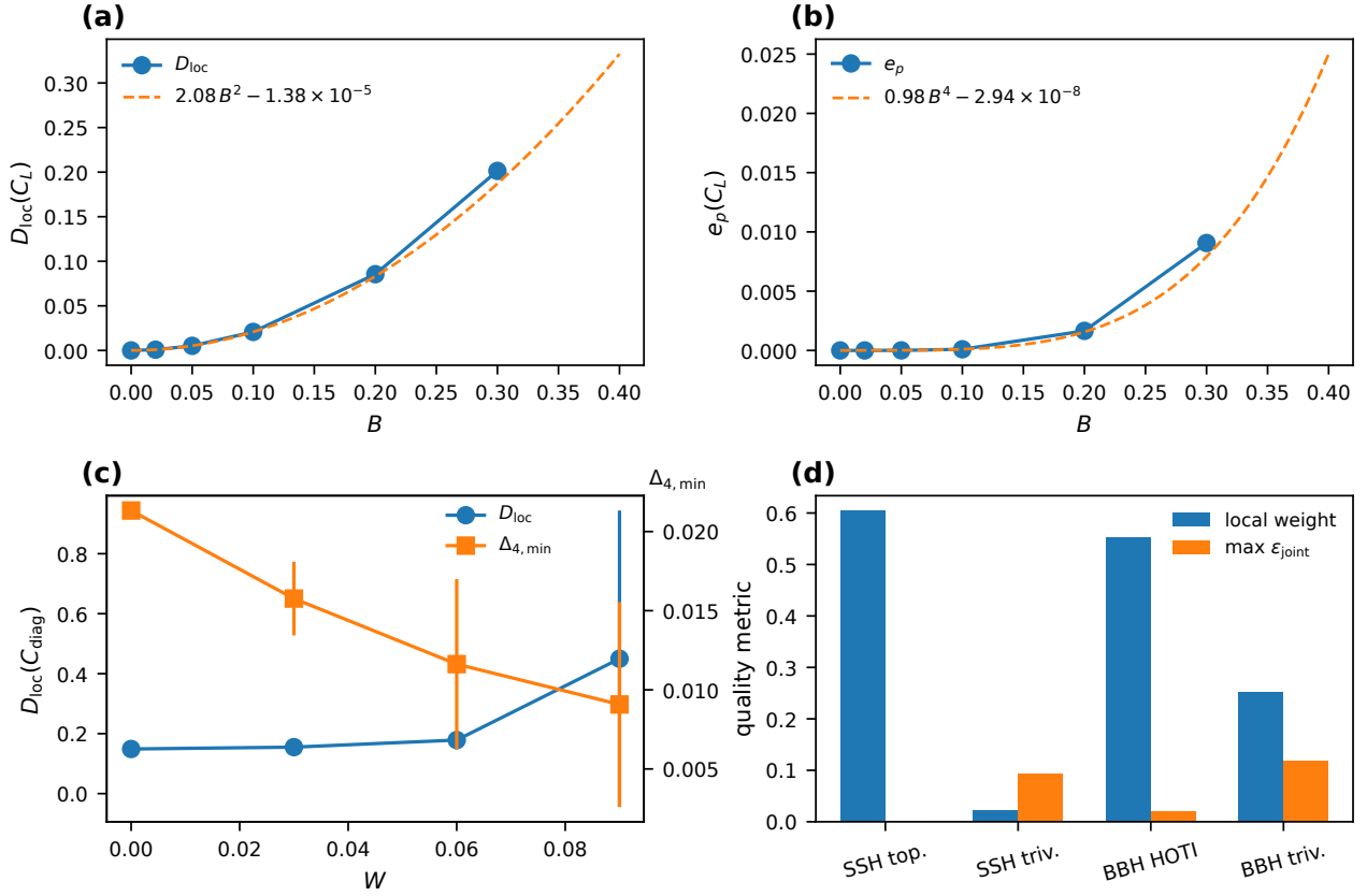
Figure 9. Additional controls. (a,b) SSH small- B scan. The response follows quadratic scaling in D_{\text{loc}} and quartic scaling in e_p for weak driving. (c) BBH disorder scaling: a controlled regime persists for weak disorder before quartet degradation sets in. (d) Trivial dimerization and non-HOTI controls fail the quartet-quality prerequisites, showing that the benchmark requires a localized topological multiplet.
