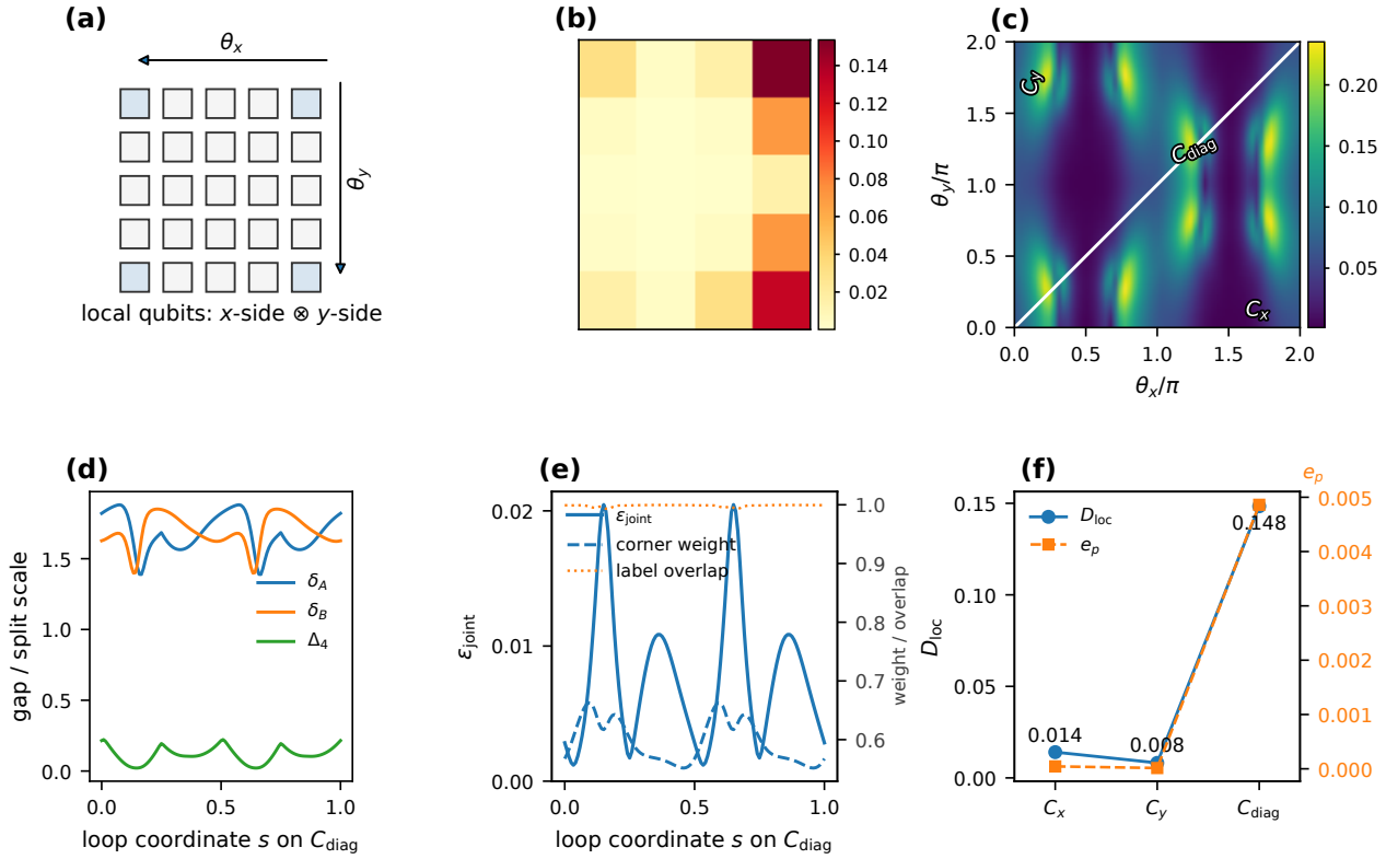
Figure 4. BBH benchmark. (a) Open BBH lattice with the corner-field torus (\theta_x, \theta_y) . (b) Representative corner-mode density at (0, 0) ; over the full torus the corner weight stays above 0.49. (c) Map of the link-level distance to the local Lie algebra, with axis and diagonal loops overlaid. (d) Along the diagonal loop the quartet gap and split diagnostics remain open. (e) The same loop keeps \epsilon_{\text{joint}} small while corner weight and label overlap remain high. (f) Loop comparison. The axis loops are almost local, while the diagonal family is entangling; the anti-diagonal family is symmetry related and agrees within the numerical resolution shown.
