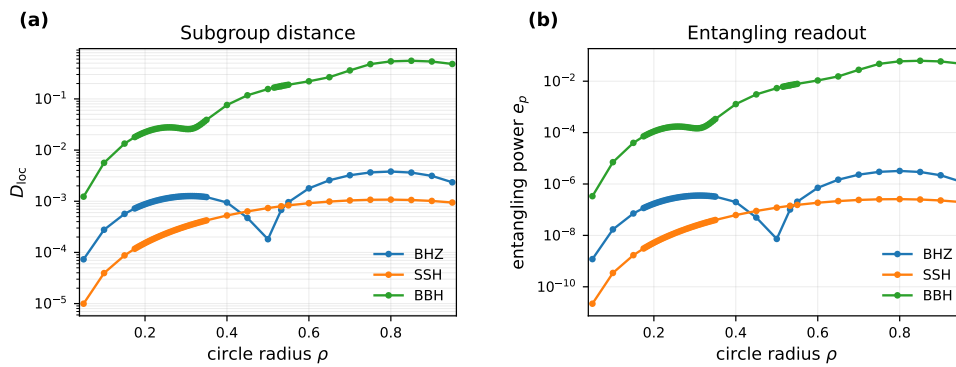
Figure 7. Radius dependence of contractible-loop nonlocality. The plotted values use the positive orientation. The reverse orientation gives the inverse holonomy and the same D_{\text{loc}} and e_p to numerical precision.
