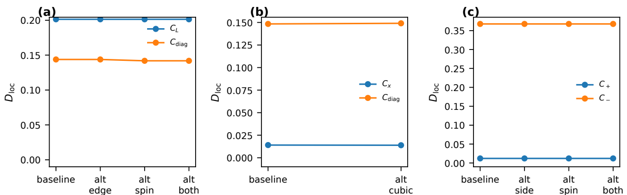
Figure 8. Observable-choice robustness. (a) SSH under coarse edge and rotated spin-like observables. (b) BBH under cubic coarse position observables. (c) BHZ under side-smoothing and rotated spin-like observables. In every case the qualitative loop-dependent pattern remains unchanged.
