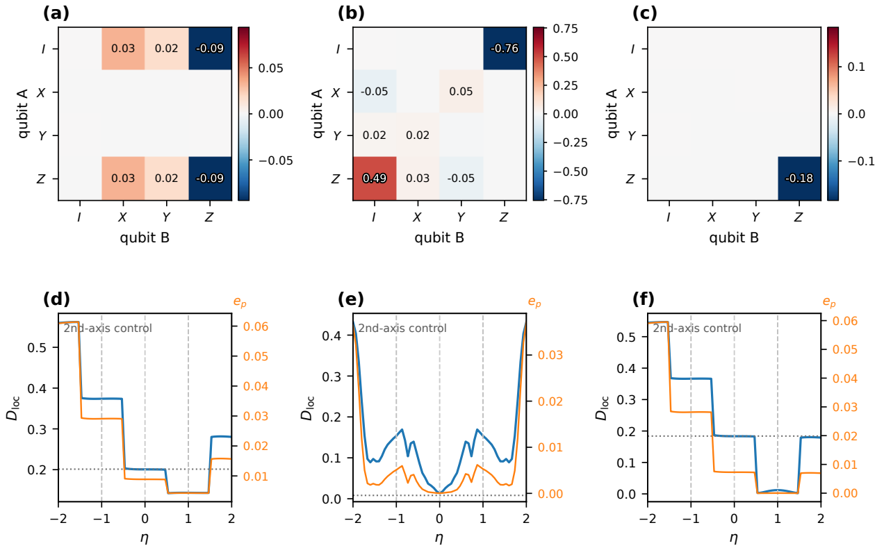
Figure 5. Mechanisms and continuous loop families. (a) Effective generator coefficients for the SSH left loop, dominated by a controlled-rotation form. (b) Effective generator coefficients for the BBH diagonal loop, with weight distributed across several higher-order channels. (c) Effective generator coefficients for the BHZ counter-rotating loop, dominated by the edge-helical Ising channel Z_{\text{edge}} \otimes Z_h ; the panel notation Z_K denotes the same helical-pseudospin factor. (d-f) Continuous scans of (\theta_1, \theta_2) = (t, \eta t) over \eta \in [-2, 2] . For non-integer \eta , the path is closed by a short return segment. The blue curve shows D_{\text{loc}} , the orange curve shows entangling power e_p , dotted horizontal lines denote the second-axis control, and dashed vertical lines mark \eta = -1, 0, 1 . These scans show connected branches in slope space rather than an optimization over all closed loops at fixed slope.
