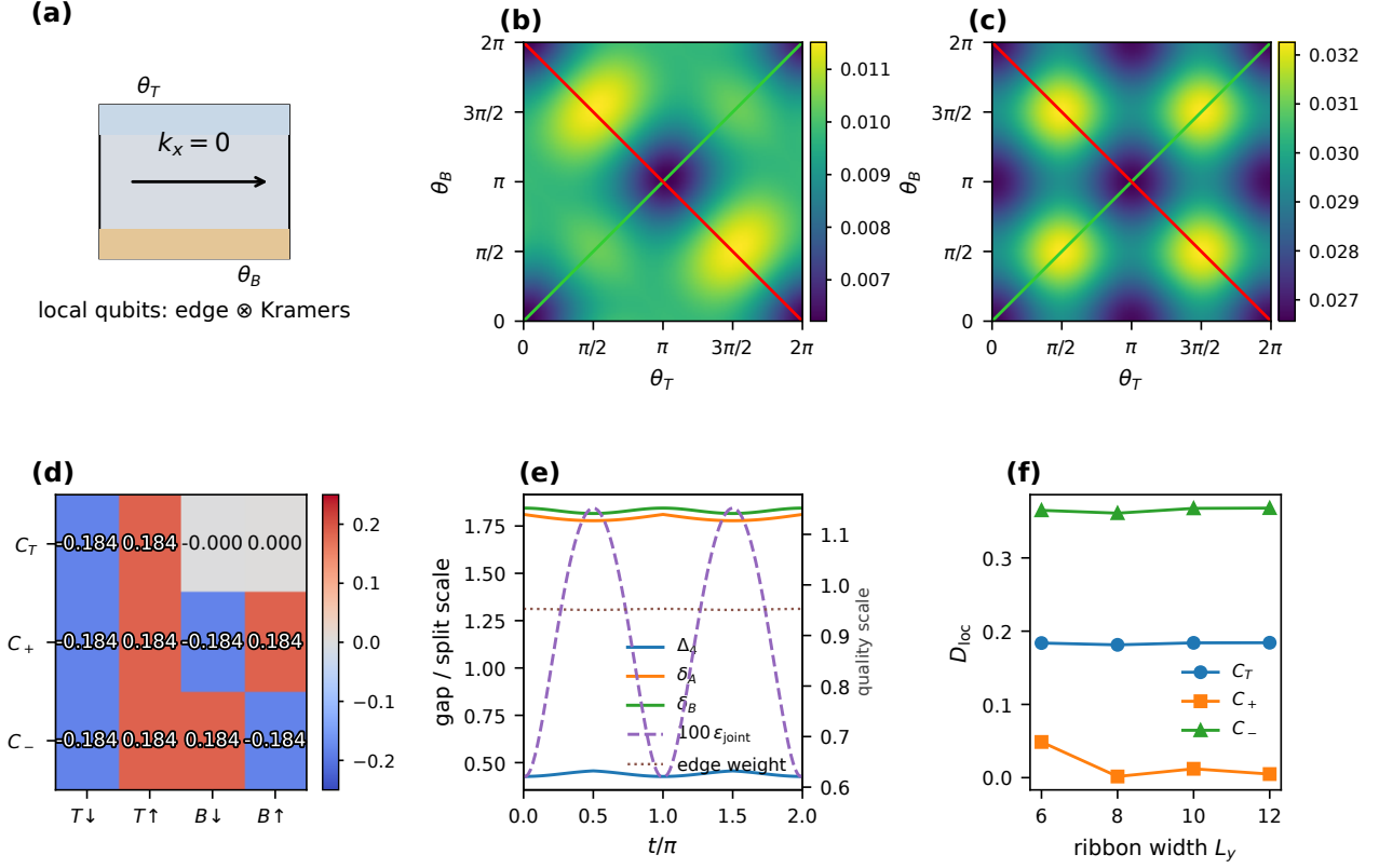
Figure 1. BHZ ribbon benchmark. (a) Ribbon slice with independent top and bottom edge angles ( \theta_T, \theta_B ). (b) Pointwise \epsilon_{\text{joint}} map on the edge-angle torus. (c) Link-level distance to the local Lie algebra. (d) Phase pattern of the counter-rotating holonomy in the extracted basis [T \downarrow, T \uparrow, B \downarrow, B \uparrow] ; the panel’s “Kramers” label denotes the time-reversal-symmetric ancestry of the extracted helical pseudospin factor. (e) Along-loop quality on C_- . (f) Width dependence: the counter-rotating response remains finite within the benchmark family while the co-rotating control stays near local.
